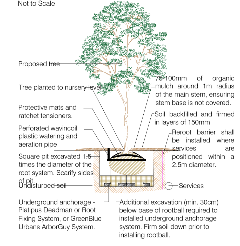
Detail 1: Tree Planting Underground Guying Not to Scale
