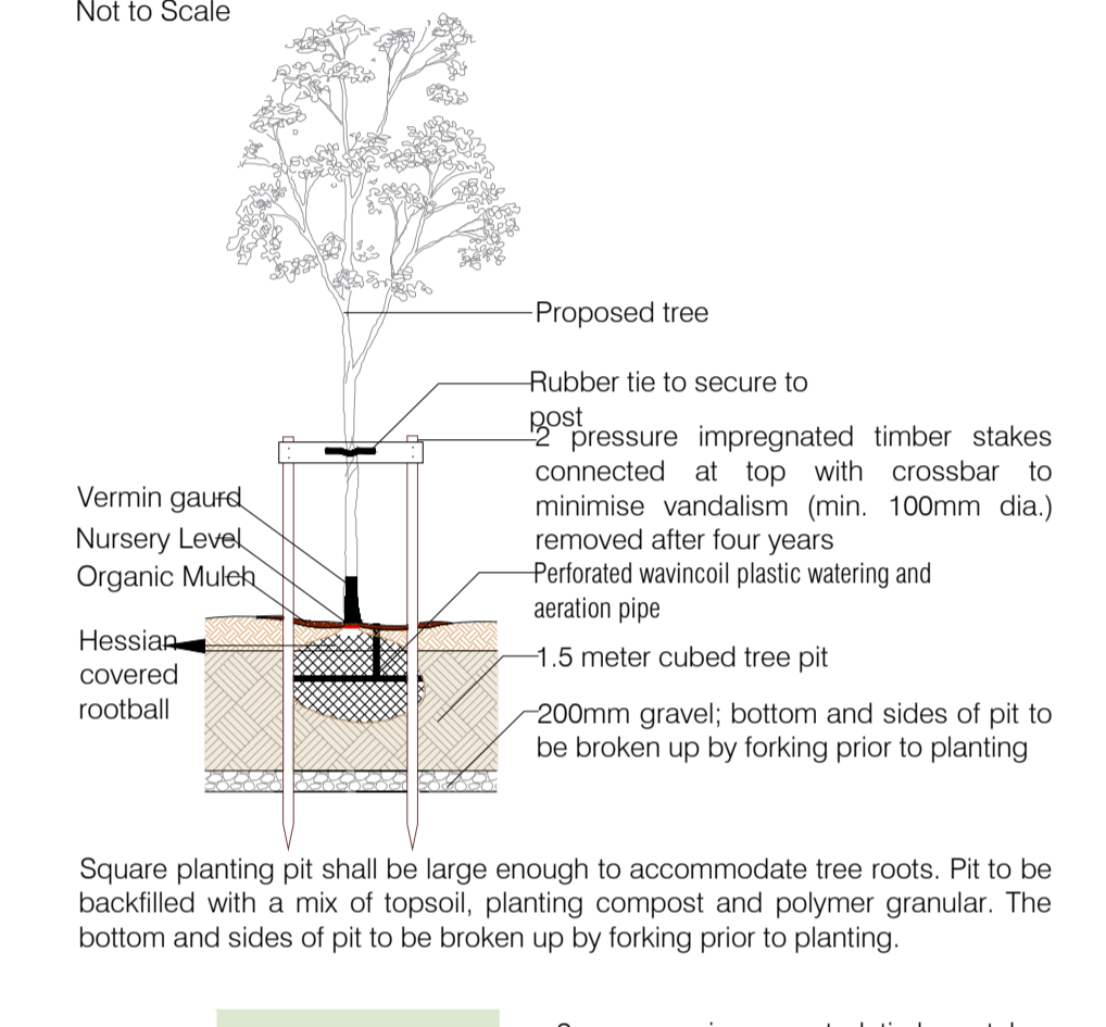
Detail 2: Standard Rootball Tree Planting Specification Not to Scale
